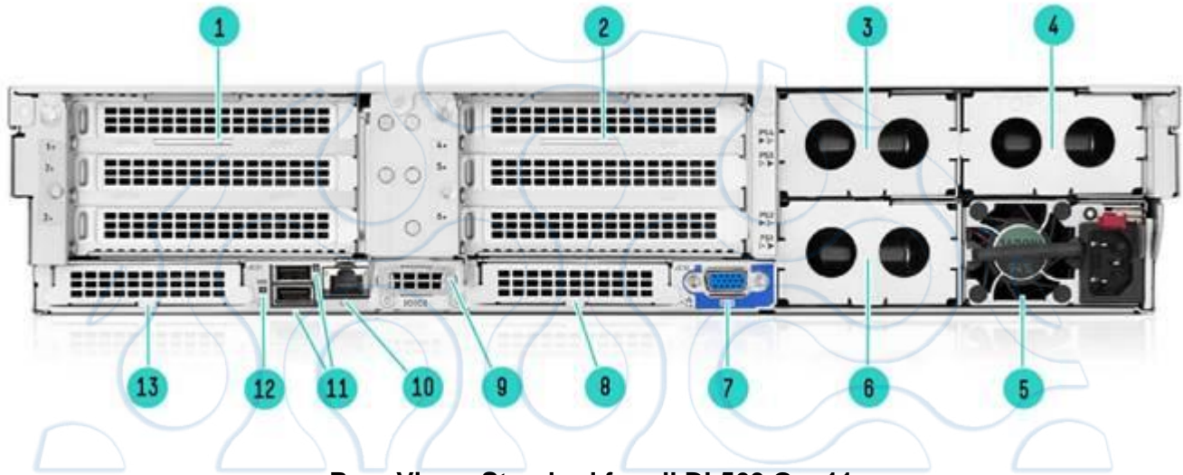
Rear View - Standard for all DL560 Gen11
