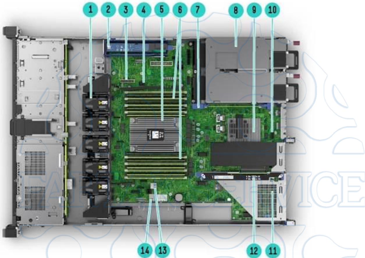
Internal View 8SFF chassis -with optional FlexLOM, Smart array shown
