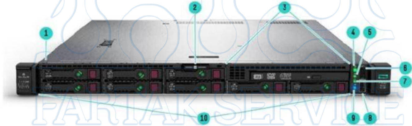
8SFF Front View - 8SFF + ODD Shown
