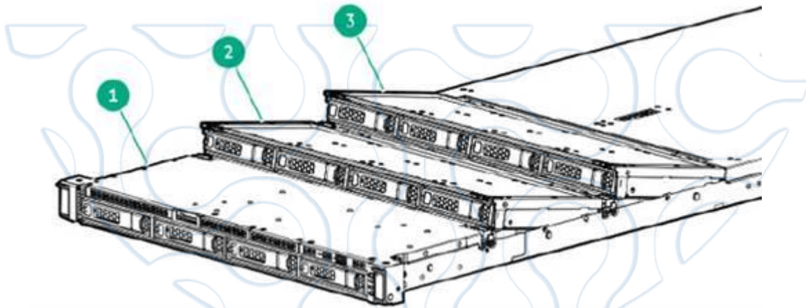
12 SFF drive bay positioning
