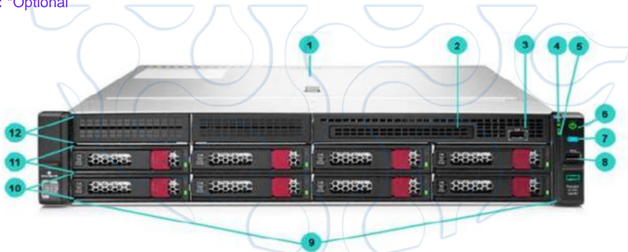
8LFF Chassis - Front View
